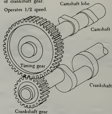
FIGURE 1-21. Cam drive mechanism opposed-type aircraft engine.
